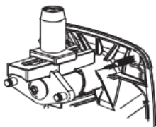
Adjustable three point roller cam
